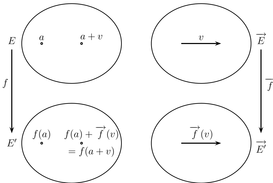
Figure 2.12: An affine map f and its associated linear map \overrightarrow{f}
